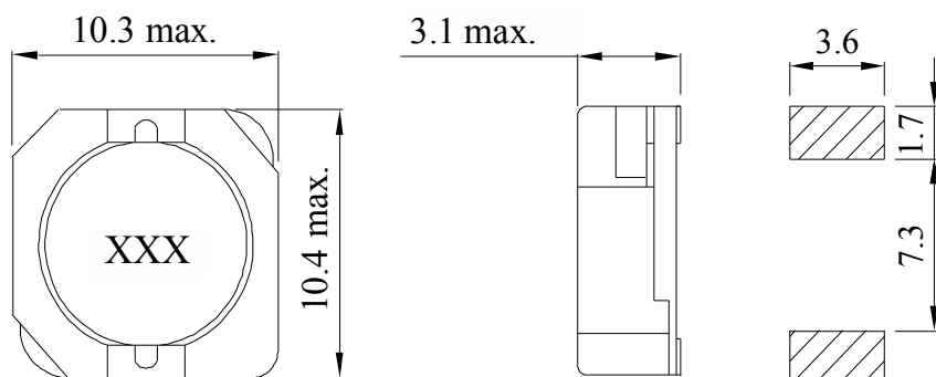
Land Pattern
